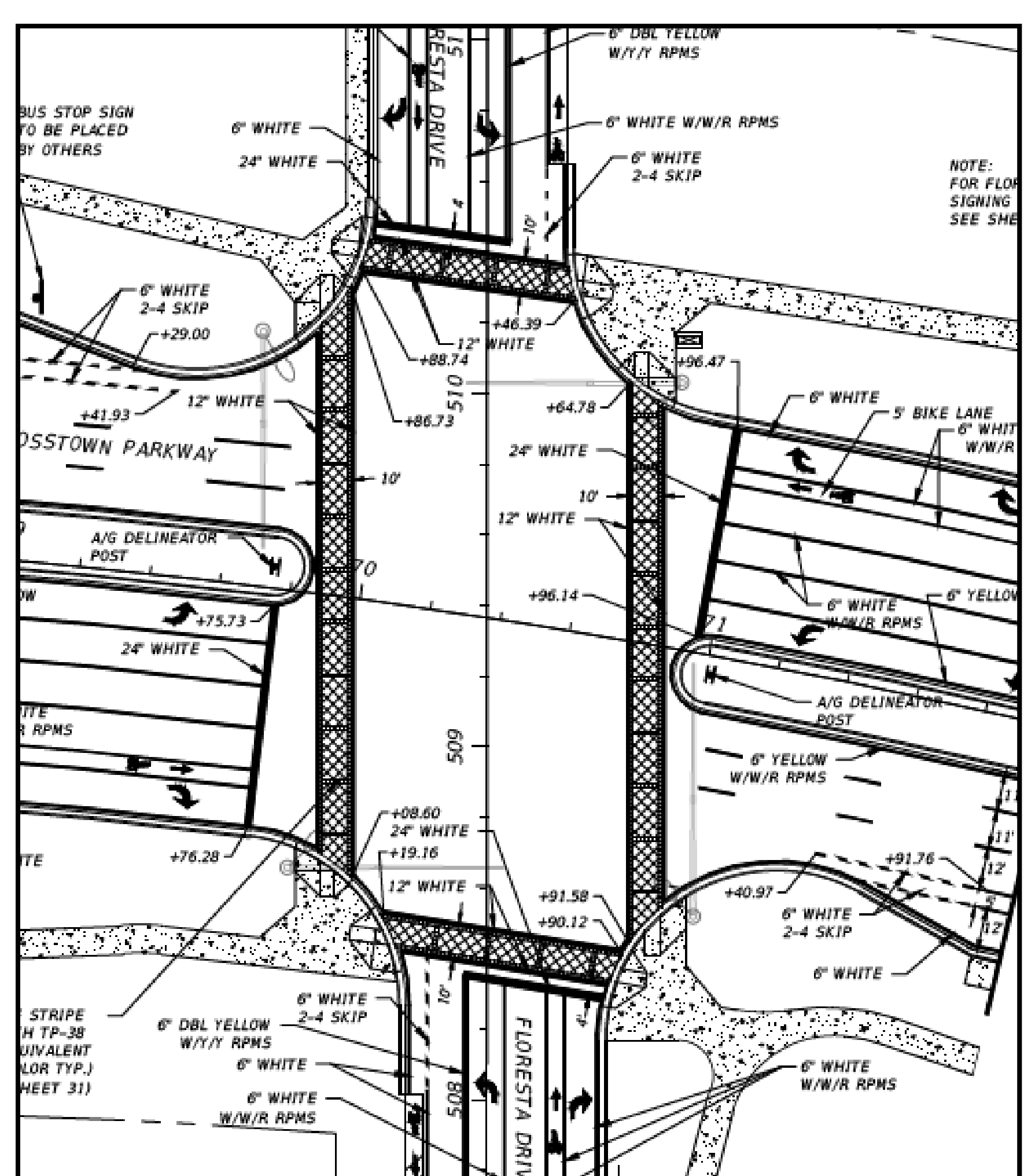
Traditional Intersection
