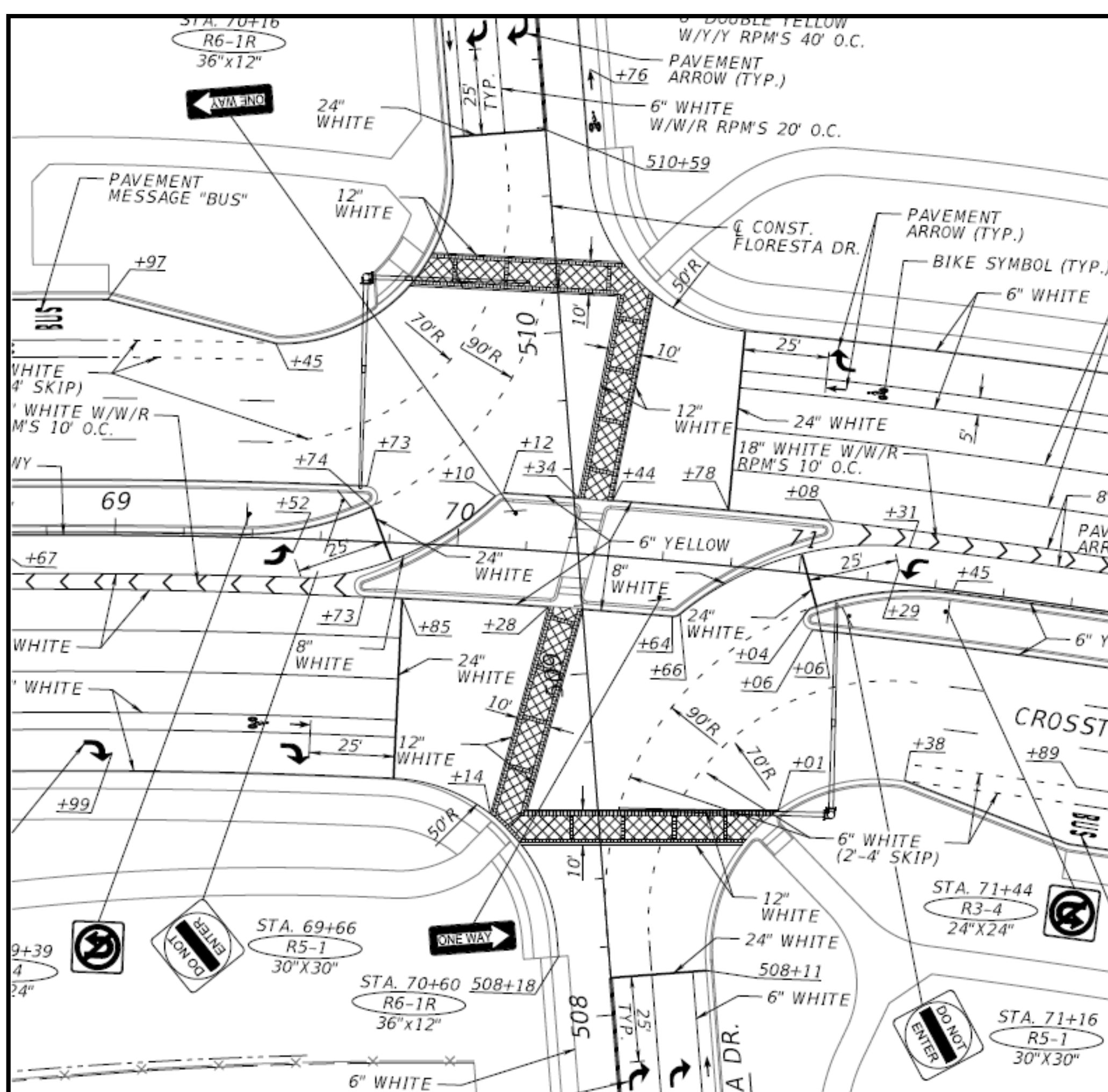
Superstreet Intersection
